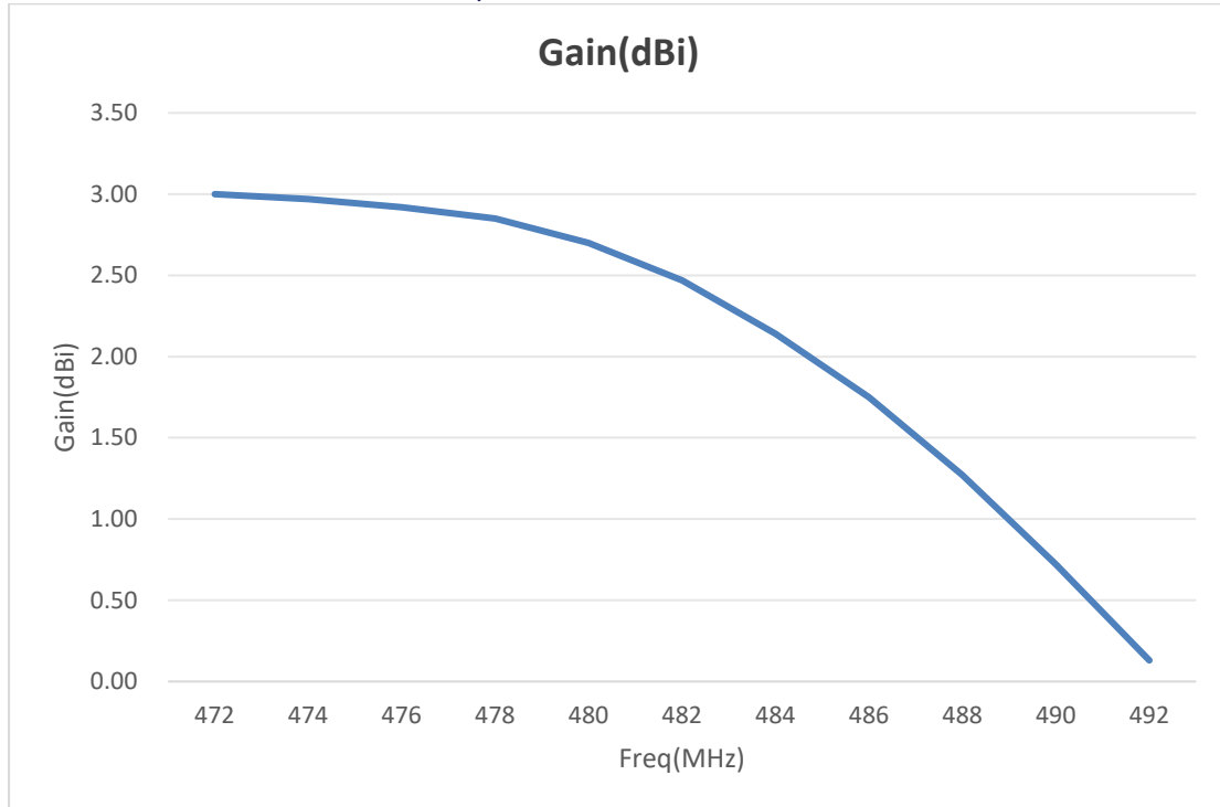
Peak Gain (dBi / Welded on 100*28mm PCB board)
