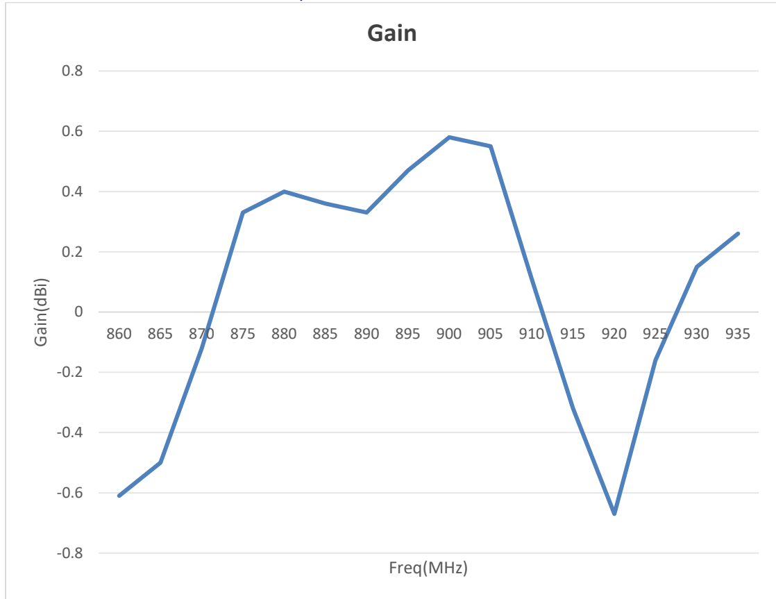
Peak Gain (dBi / Welded on 100*28mm PCB board)
