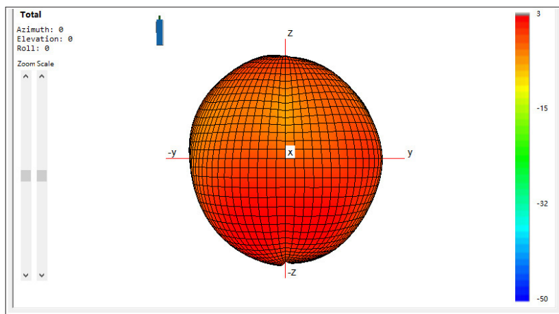
ANT 1 3D radiation patterns @ 5500 MHz
