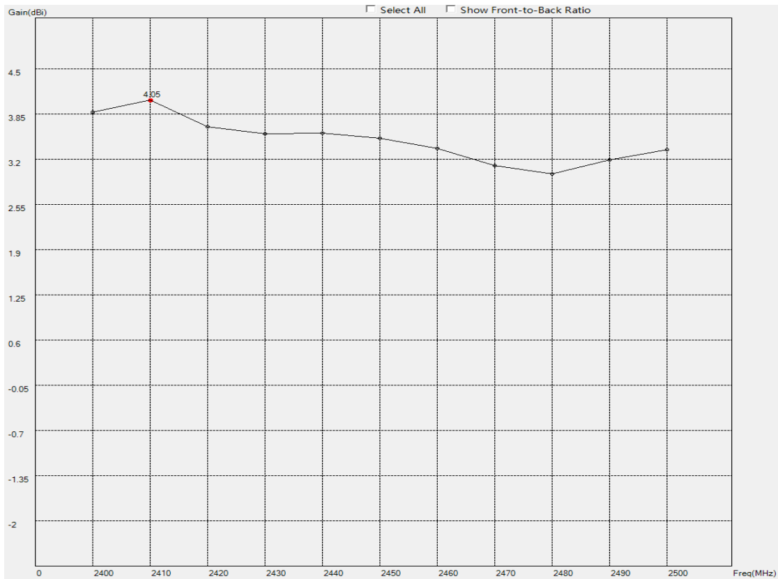
Peak Gain (dBi, Bending state)
