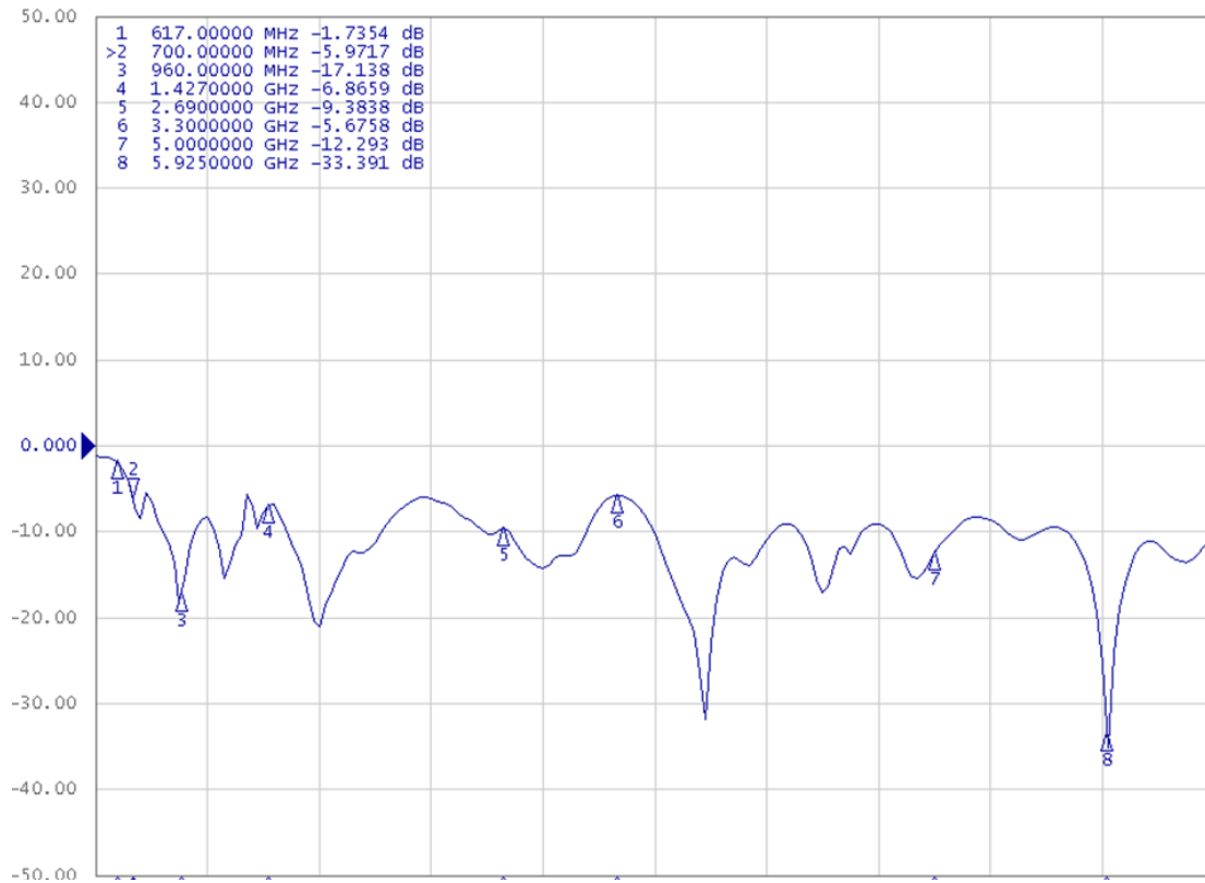
Return Loss
